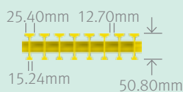
Elevation View
