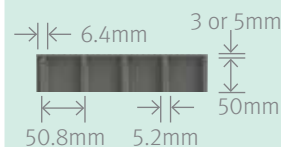
Elevation View
