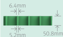
Elevation View
