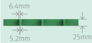
Elevation View
