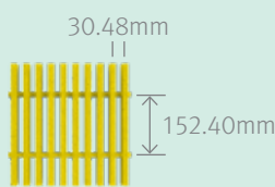
Plan View
