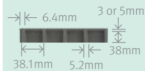
Elevation View
