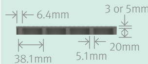
Elevation View
