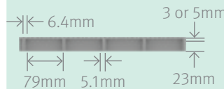
Elevation View
