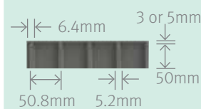
Elevation View
