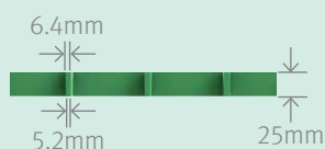
Elevation View
