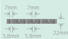
Elevation View
