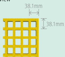
Plan View
