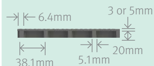
Elevation View
