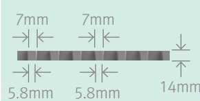
Elevation View
