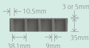
Elevation View
