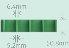
Elevation View
