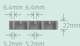
Elevation View
