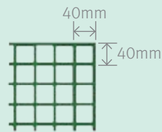
Plan View
