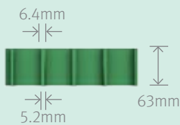
Elevation View
