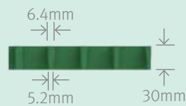
Elevation View
