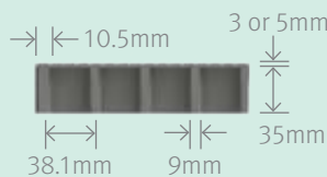
Elevation View
