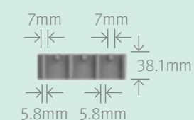
Elevation View
