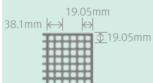
Plan View
