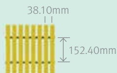
Plan View
