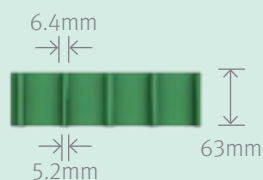
Elevation View
