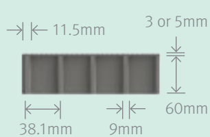
Elevation View
