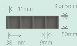
Elevation View
