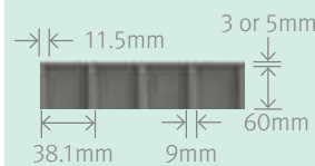
Elevation View
