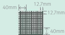
Plan View
