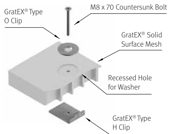
OH Clip Assembly
