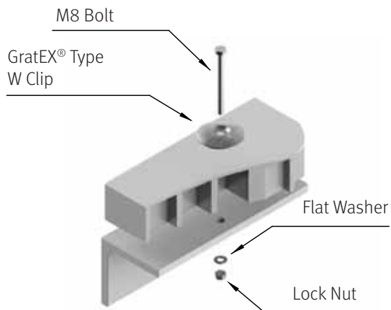
W Clip Assembly
