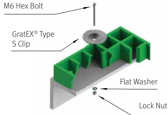
S Clip Installation Tool
