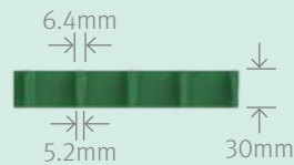
Elevation View
