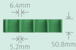
Elevation View
