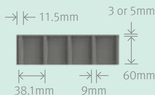
Elevation View
