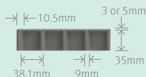
Elevation View
