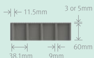
Elevation View
