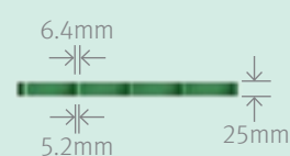
Elevation View
