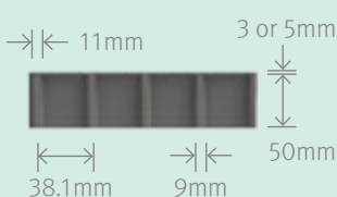
Elevation View
