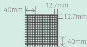
Plan View
