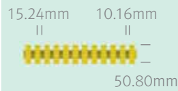
Elevation View
