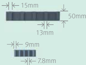
Elevation View
