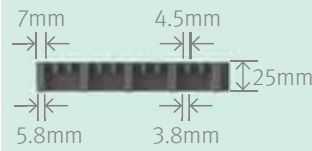
Elevation View
