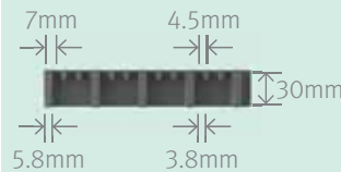
Elevation View
