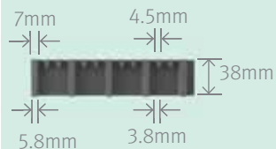
Elevation View
