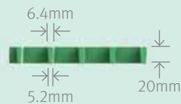
Elevation View
