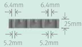
Elevation View
