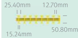
Elevation View
