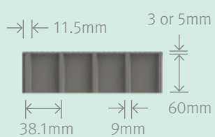
Elevation View
