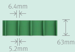
Elevation View
