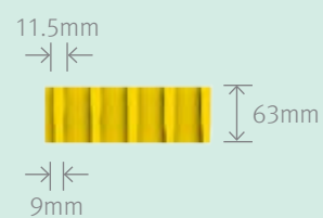
Elevation View
