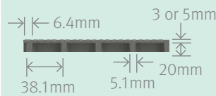
Elevation View
