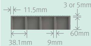
Elevation View
