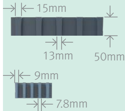
Elevation View
