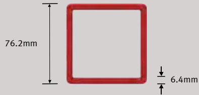
76.2 x 76.2 x 6.4mm Square Hollow Section
