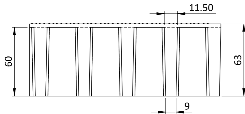
ELEVATION VIEW
