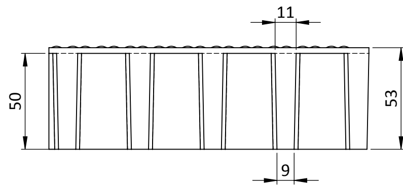
ELEVATION VIEW
