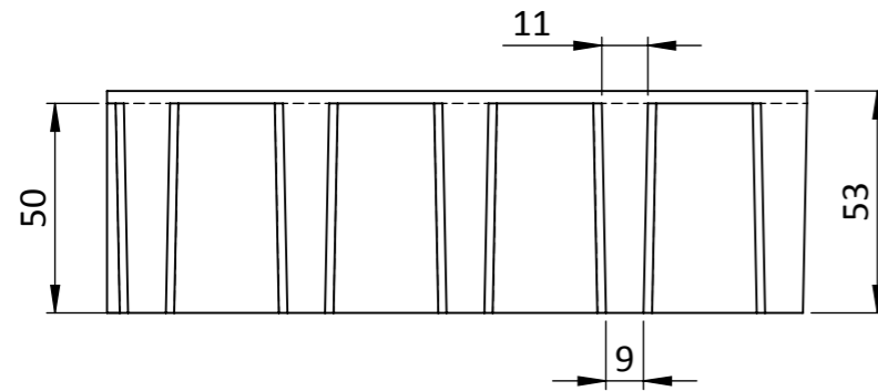
ELEVATION VIEW
