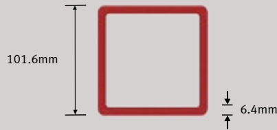
101.6 x 101.6 x 6.4mm Square Hollow Section
