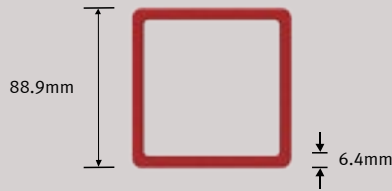
88.9 x 88.9 x 6.4mm Square Hollow Section
