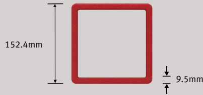
152.4 x 153.4 x 9.5mm Square Hollow Section
