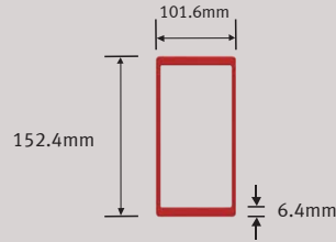
152.4 x 101.6 x 6.4mm Rectangular Hollow Section
